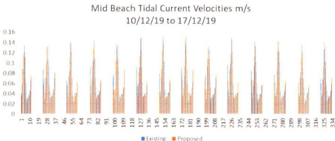
Figure 18: Mid Beach, tidal currents existing and with proposed development
