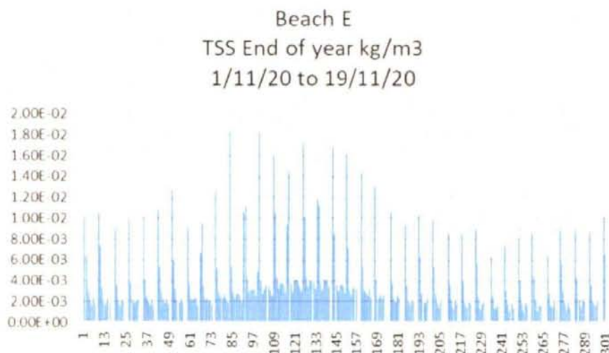
Figure 20 : Suspended sediment concentrations at the east beach location
