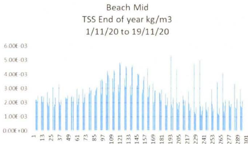
Figure 21: Suspended sediment concentrations at the mid beach location
