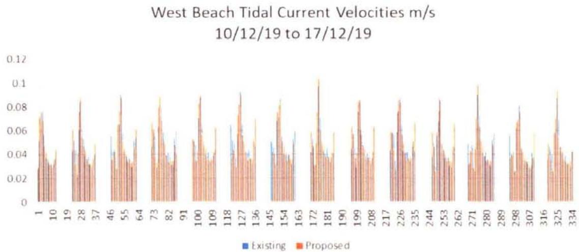
Figure 19: West Beach, tidal currents existing and with proposed development
