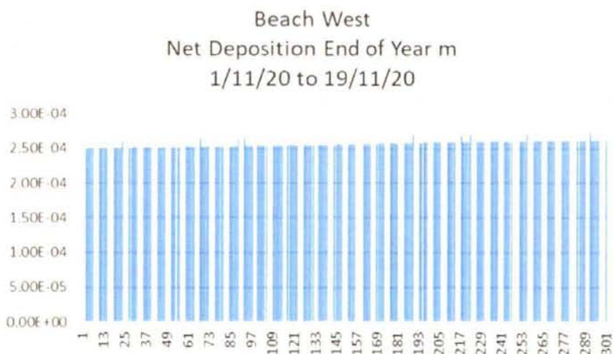
Figure 25 Beach West, Net deposition existing situation
