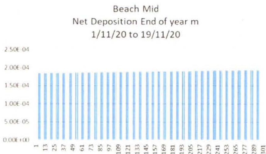
Figure 24 Beach Mid, Net deposition existing situation
