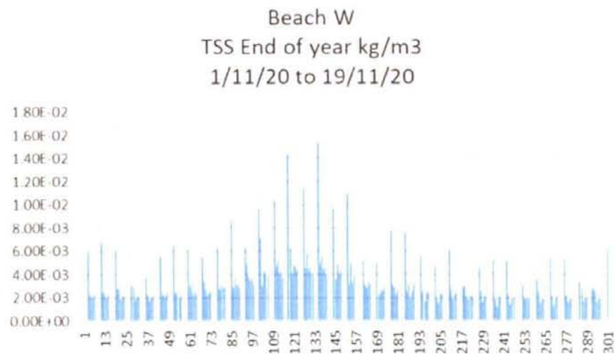
Figure 22: Suspended sediment concentrations at the west beach location
