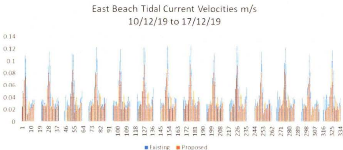
Figure 17: East Beach, tidal currents existing and with proposed development
