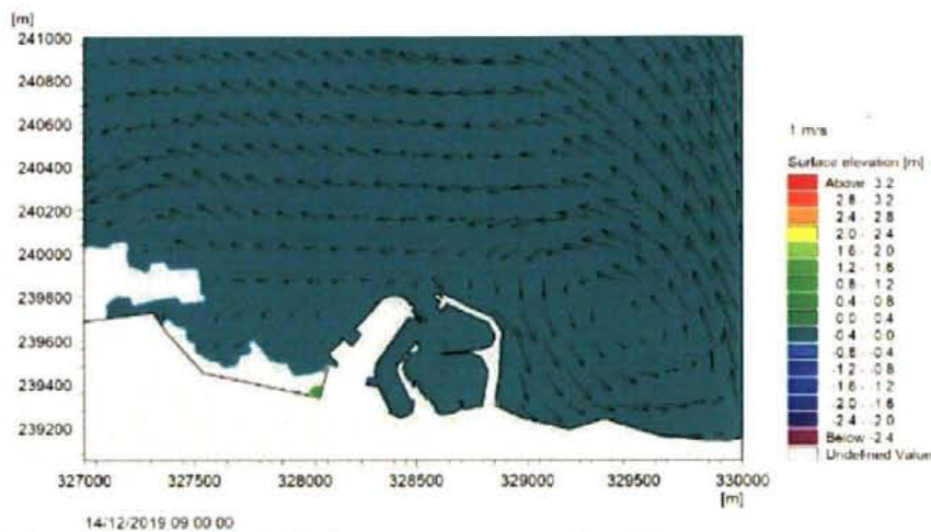
Figure 15: Mid Flood Tidal Currents, Proposed Works
