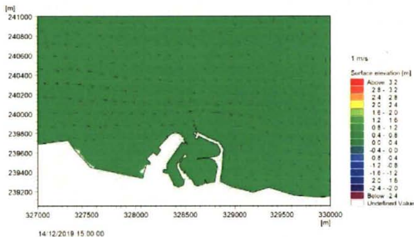
Figure 16: Mid Ebb Tidal Currents, Proposed Works
